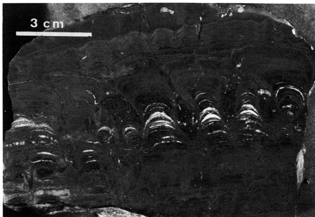
Fig. 7. "Deep water" stromatolite from condensed iron-stained cephalopod limestone. Upper Famennian, Tizi Bou Kerzia, Mader Platform. Polished slab.
