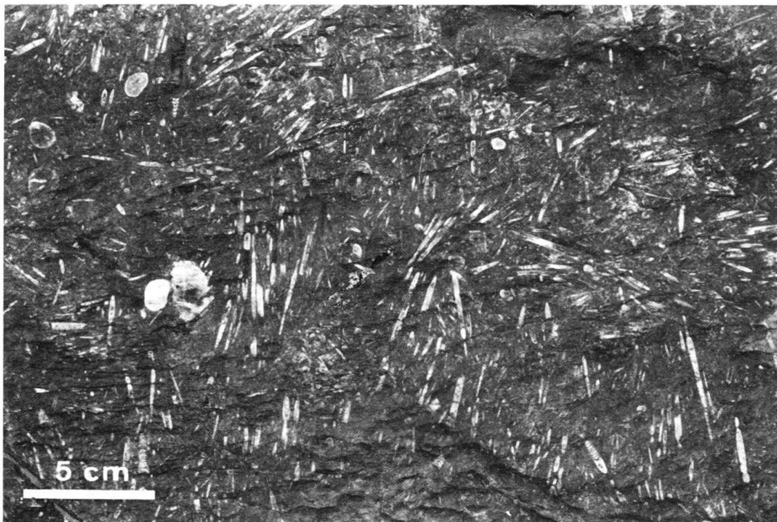
Fig. 10. Accumulation of small orthoconic nautiloids on a bedding plane of uppermost Frasnian black cephalopod limestone. Jebel Amelane, Tafilalt Platform.
