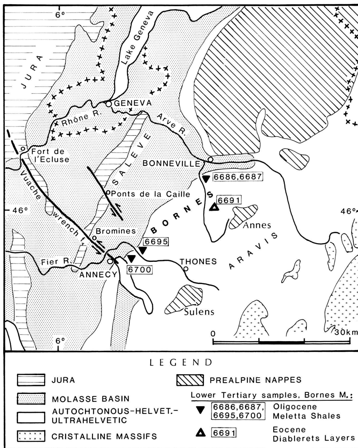
Fig. 8. Location of selected Lower Tertiary samples in the Bornes Massif (see Table 2 for coordinates). The higher maturity (see Table 4) of samples 6686, 6687 and 6691 to the east may reflect the overburden of the now-eroded prealpine nappes. Immature samples 6695 and 6700 to the west are located in the vicinity of a regional wrench fault zone, the reactivation of which may have resulted in short episodes of high heat flow affecting some geochemical parameters of the samples.
