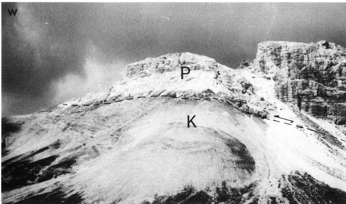
Fig. 5. The Puez thrust, with Norian Dolomia Principale (P) in the hangingwall and the Lower Cretaceous Puez Marls (K) in the strongly sheared footwall. Puez Massif, central-northern Dolomites. The thrust is almost flat and it is WSW-directed, Paleogene in age, and belonging to the Dinaric thrust belt front. Compare Fig. 4.
