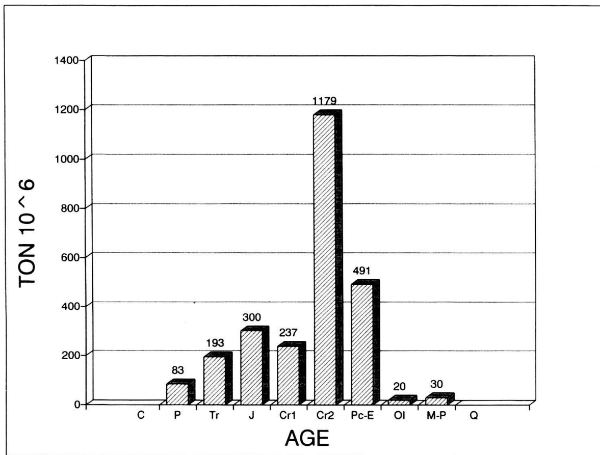
Fig. 19. Tonnage versus time of Phanerozoic Mediterranean karst bauxites, in 10^6 tons (data from Bárdossy 1982).
