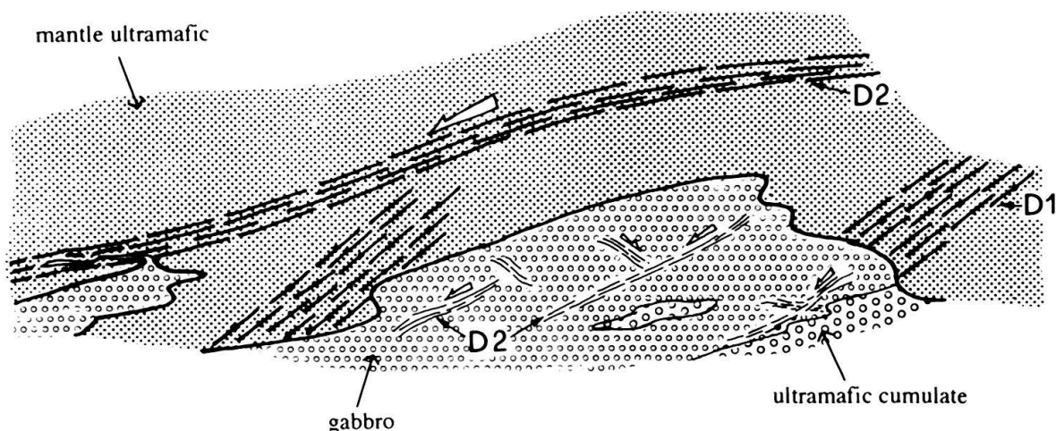
Fig. 5. Idealized and schematic representation of the earliest deformation geometries based on the interpretation of field data in the Bracco area.
