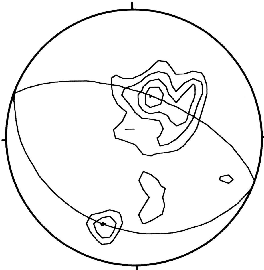
Fig. 4. Plot of the overall restored foliation poles (m. 200). Two main systems are defined at 90–100° to each other, the main system dipping 20–30° towards SW (equal area projection, lower hemisphere contours at 2–3 etc. times unit).
