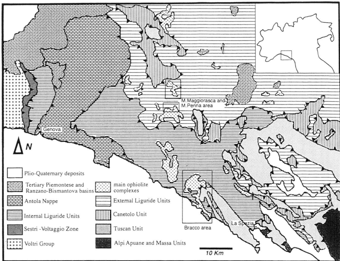
Fig. 1. Geological sketch map of the Northern Apennine with location of the areas quoted in the text.
