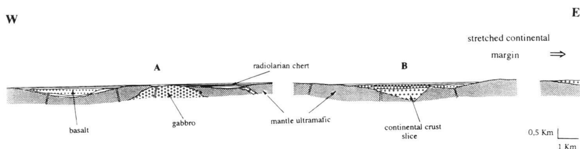
Fig. 7. Schematic representation of the Ligurian Domain as derived by field relationships in the Northern Apennine ophiolites. Section A derives from the Bracco area and surroundings (Internal Ligurides), whereas section B from field evidence in the Ligurian/Emilian Apennine (External Ligurides).
