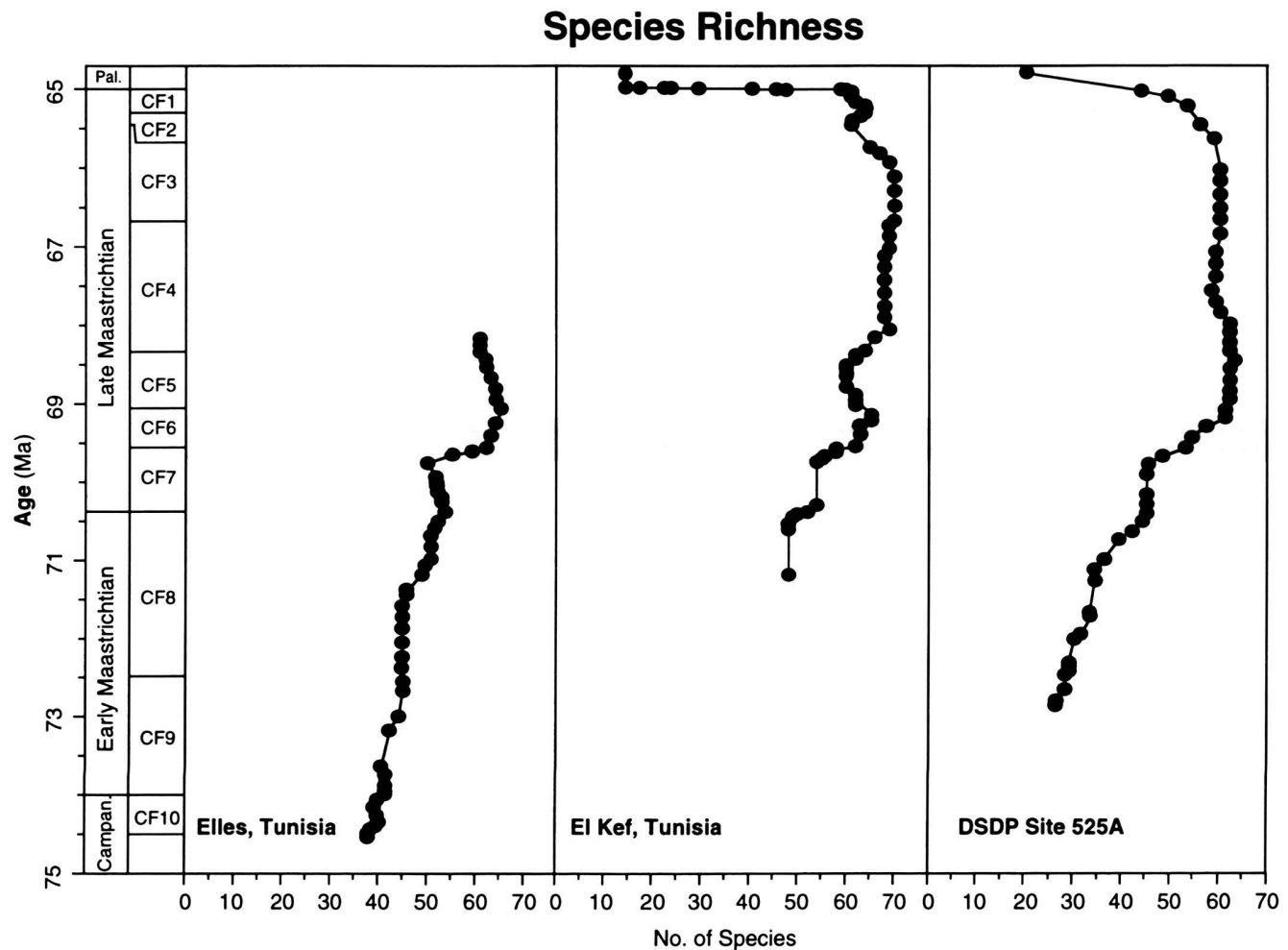
Fig. 7. Maastrichtian species richness in planktic foraminifera of low (El Kef and Elles) and middle latitudes (Site 525A). Note that maximum species richness was attained rapidly during a short period of only about 600 kyr. The mass extinction of planktic foraminifera also occurred very rapidly during the last 400 kyr of the Maastrichtian.
