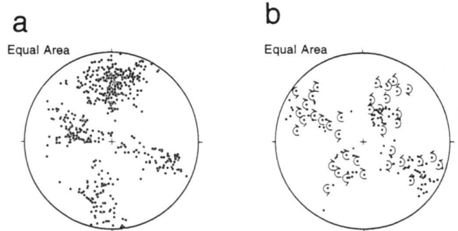
Fig. 11. (a) Poles of cleavage in the Lech Formation. The cleavage displays two maxima: the main maximum is oriented at around 100/78 SSW and a secondary maximum at around 25/80 WNW and 25/80 ESE. Field relationships indicate that the NNE-striking cleavage was modified and rotated during the development of the ESE-striking cleavage. (b) Stereoplot of fold axis of small-scale folds and sense of vergence (shown as rotation axes looking down the plunge) in the Lech Formation. The locally observed refolding of the hinge lines indicated that NE-trending small scale folds were overprinted by NW-trending small scale folds.
