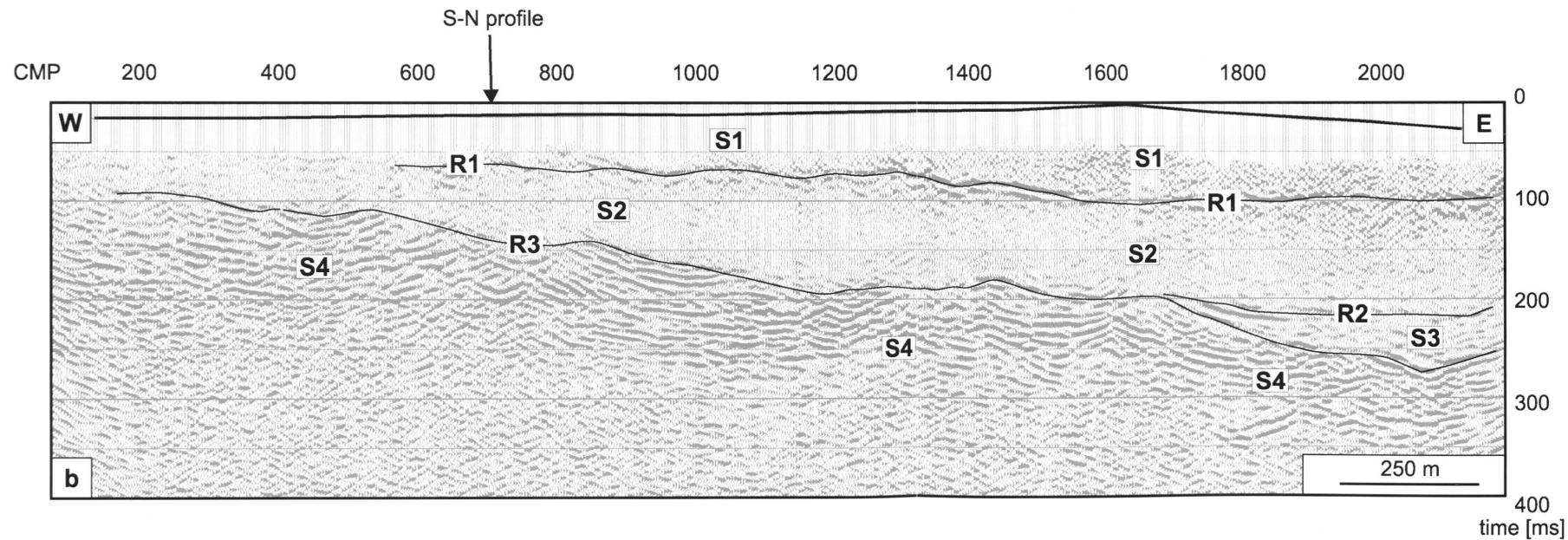
Fig. 7. (a) stacked section of Profile 2 (east-west profile). Note changes in amplitude character with two-way time as in fig. 6a. (b) Migrated section of (a) with interpreted units and main reflectors. Arrow on (b) marks the intersection with Profile 1 (S-N profile). For identification of units see text and Fig. 8.
