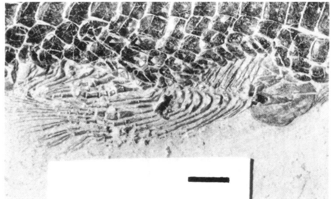
Fig. 20: Peltoperleidus bellipinnis BÜRGIN, 1992 (Balken 2 mm). Analis in Lateralansicht (PIMUZ A/I 2664, Ducanfur- ga 4, Sertig, Davos).
