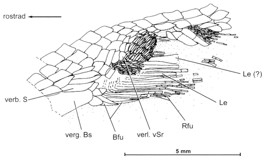
Fig. 15: Peltopterus ducanensis BÜRGIN et al., 1991. Anals in Lateralansicht (PIMUZ A/I 3314, Ducanfurrga 3, Sertig, Davos).
