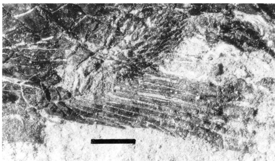
Fig. 14: Peltopterus ducanensis BÜRGIN et al., 1991 (Balken 1 mm). Anals in Lateralansicht (PIMUZ A/I 3314, Ducanfurrga 3, Sertig, Davos).
