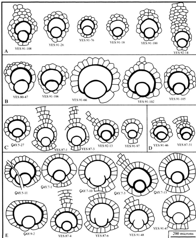
Fig. 3. Megalospheric embryo, early chamberlets and their variation in A- N. strophiolata (Gümbel, 1868) fermonii Less, 1987, B- N. evae Less, 1987, C- D. augustae van der Weijden, 1940 sourbetensis Less, 1987, D- D. trabayensis trabayensis Neumann, 1955, E- D. 'dispansa' (Sowerby, 1840) taurica Less, 1987.
