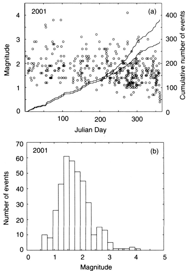
Fig. 6. Earthquake activity during 2001: magnitude of each event and cumulative number of events (a); histogram of magnitudes (b). In (a) the upper curve shows the cumulative number of all events, whereas the lower curve corresponds to the number of events without the Bormio aftershocks and the Val Baone events.
