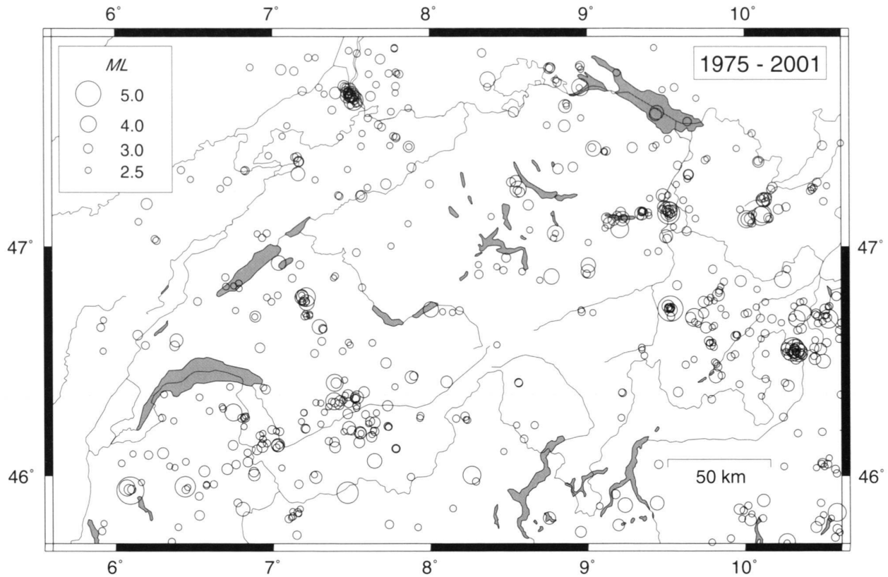
Fig. 3. Epicenters of earthquakes with Magnitudes M_L \geq 2.5 , during the period 1975–2001.
