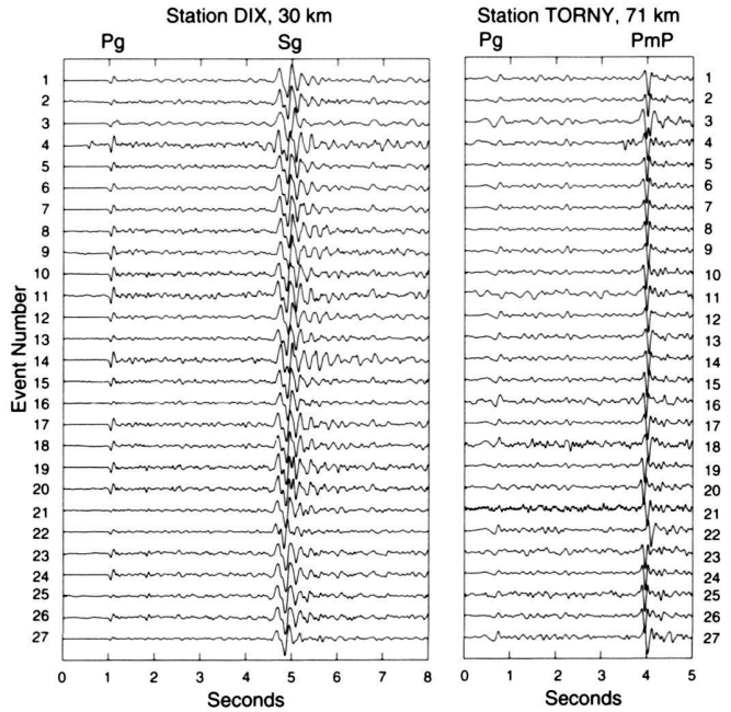
Fig. 8. Seismograms of the Martigny events recorded at stations DIX and TORNY. The signals at DIX are aligned on the Pg arrivals and bandpass filtered between 0.5 and 16 Hz; the signals at TORNY are bandpass filtered between 1 and 10 Hz and aligned on the Pg arrivals at station AIGLE, which features more impulsive onsets and which is located in practically the same direction as TORNY. The clearly visible shift between the PmP of events 20 and 22 implies that event 20 must be deeper and event 22 shallower.
