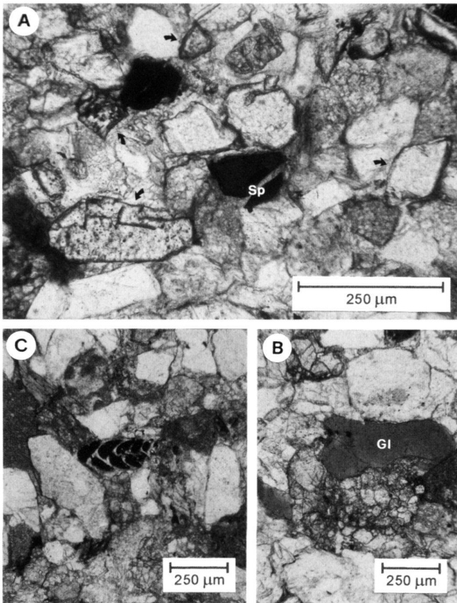
Fig. 5. Heavy minerals (A) and intrabasinal grains (B-C) in the Gonfolite sandstones of central Brianza. A) Sample DF 1 – detail on a lamina enriched in heavy minerals: garnet (arrows) and chromian spinel (Sp). B) Sample DF 9 – glaucony pellet (Gl). C) Sample DF 9 – reworked benthic foraminifer ( Brizalina sp.), with broken test and chambers filled by an oxidised matrix. All photos are in plane polarised light.
