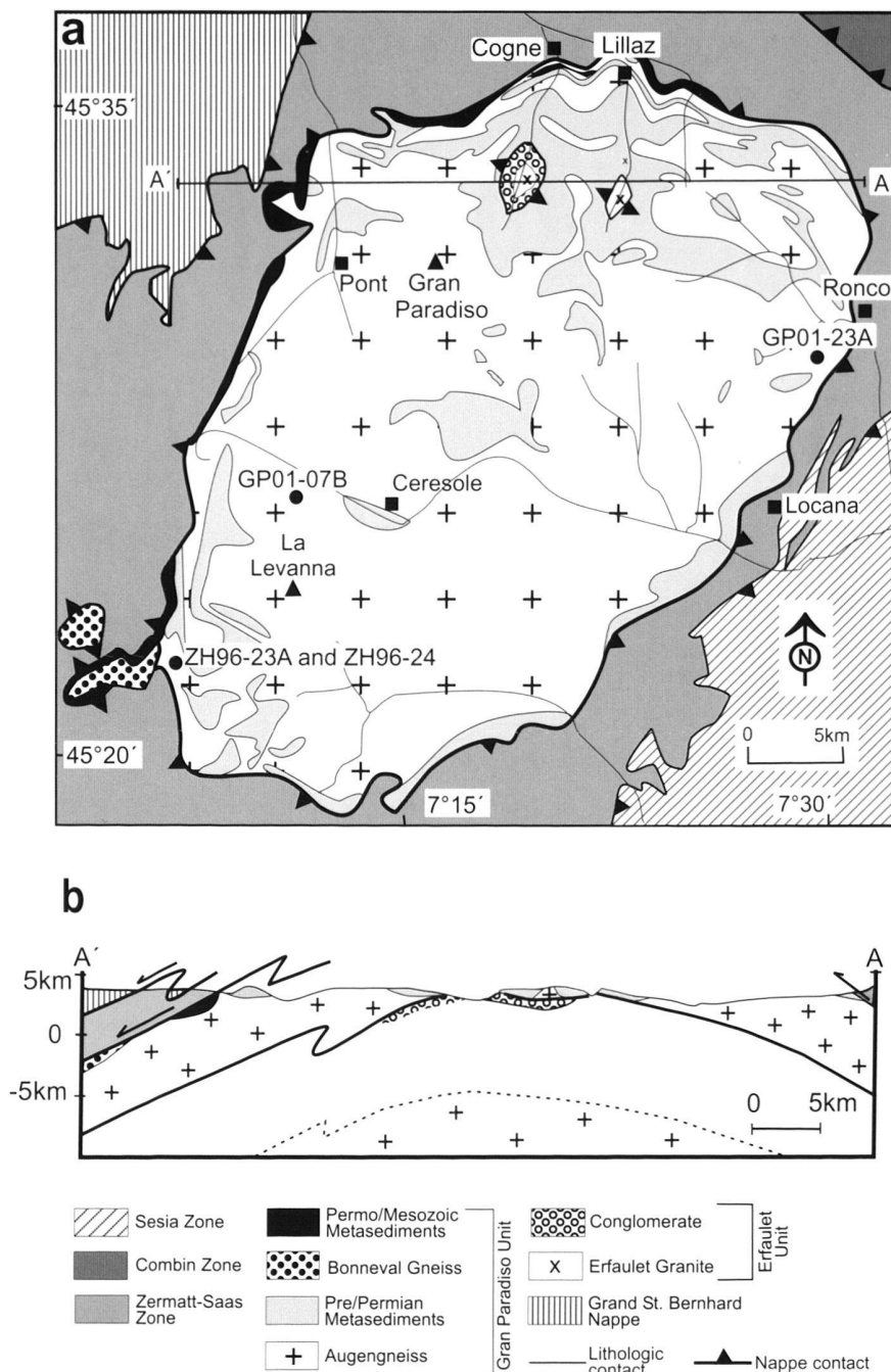
Fig. 2. (a) Tectonic map of the Gran Paradiso Massif (modified from Kassem & Ring 2004). Cross section A-A' and major streams (thin black lines) are indicated. The localities of samples GP01-7B and GP01-23A and also the sample locality of samples ZH96-23A and ZH96-24 of Bertrand et al. (2000) are indicated. (b) Cross section A-A' showing broad domal structure, the Erfaulet Unit forms the base of the exposed section and crops out in major valleys.
