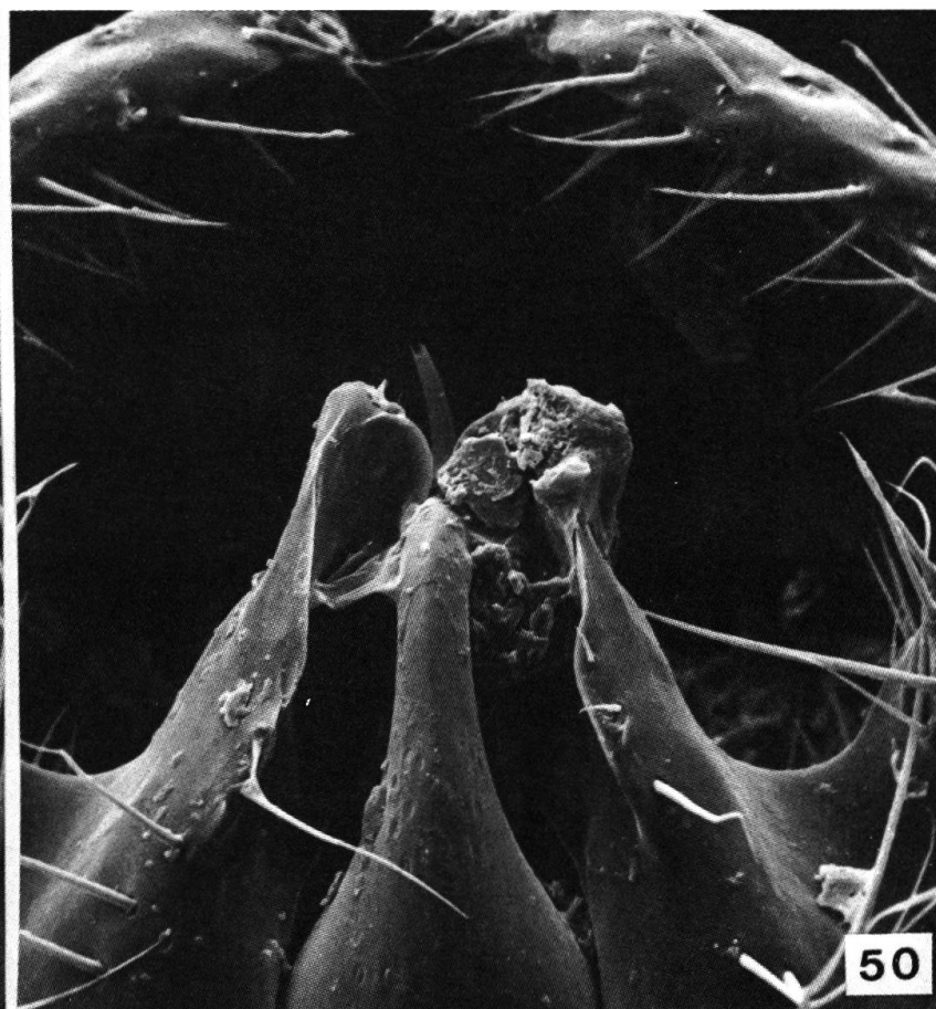
Abb. 49–50: Kopulationsapparate: 49, Malthodes pseudoparthenias n.sp. 600×. 50, Malthodes parthenias Kiesw. 600×.
