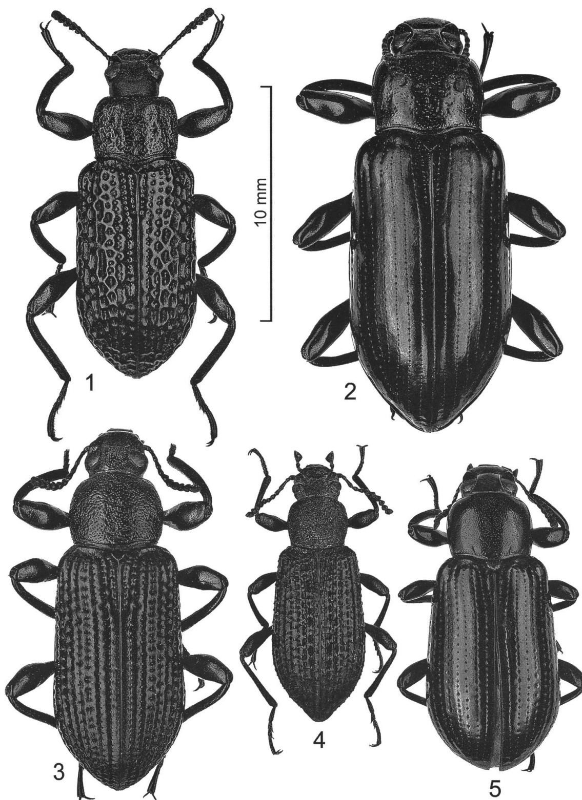
Figs 1–5. Dorsal view of the Derosphaerus species from the Nepal Himalayas: 1, D. rugosus ; 2, D. aeruginosus ; 3, D. cribrum ; 4, D. asperipennis ; 5, D. exularis .
