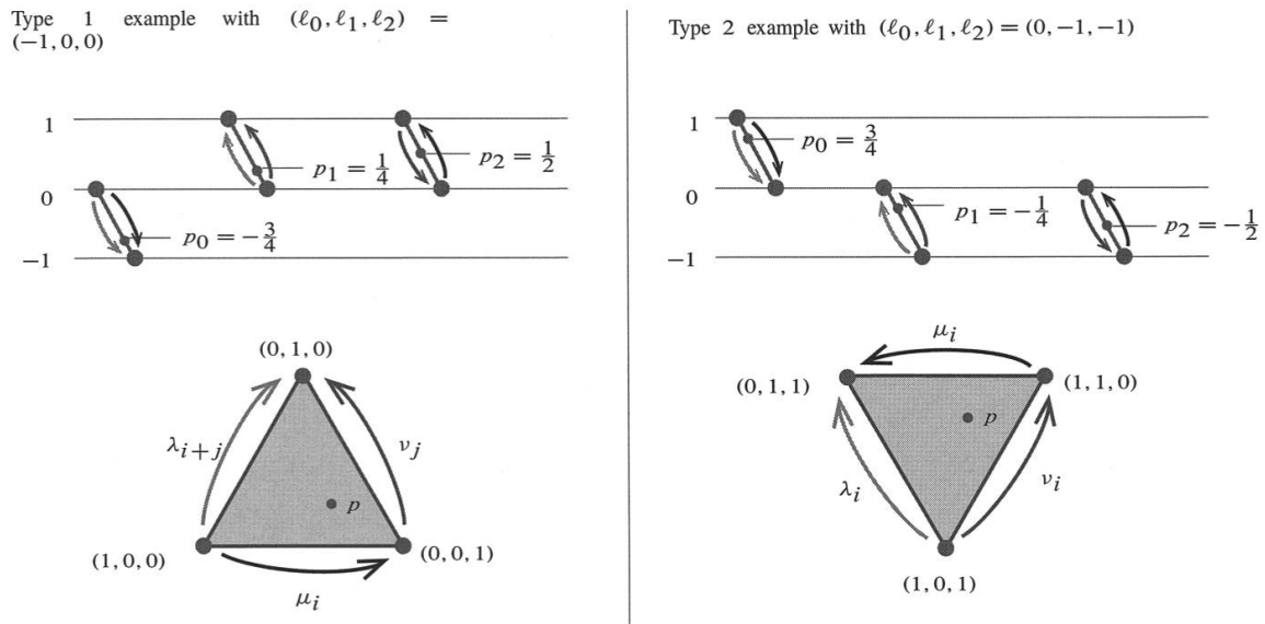
FIGURE 10 Examples of 2-cells of type 1 and 2
