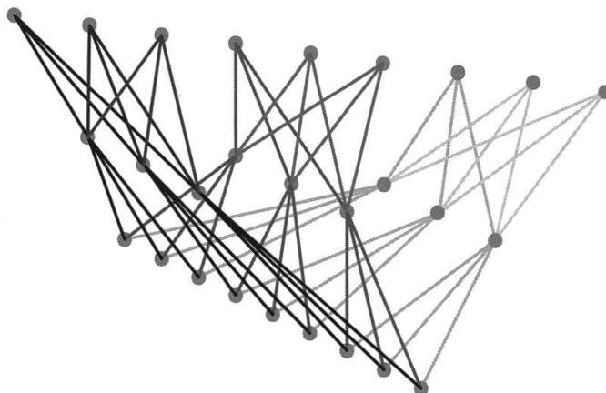
FIGURE 4 A portion of \mathcal{H}_1(\mathbb{Z}/3\mathbb{Z}) , after a figure by Dymarz in [Dym1]
