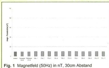
Fig. 1 Magnetfeld (50Hz) in nT, 30cm Abstand
