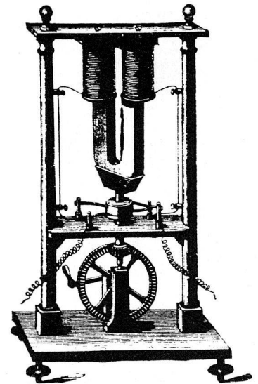
Abb. 1: Pixii's Modell, 1832.
