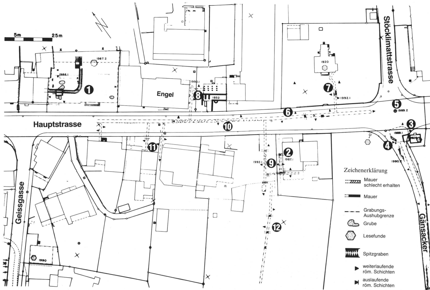
Abb. 1 Situationsplan
