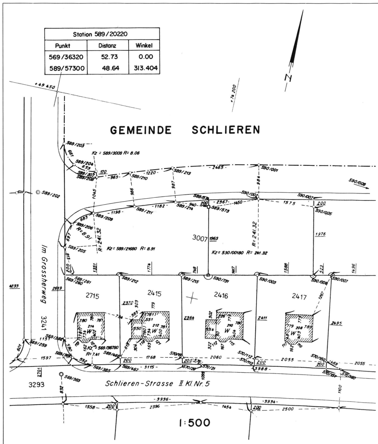
Abb. 5 Situationsplan
