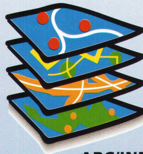
ARC/INFO
