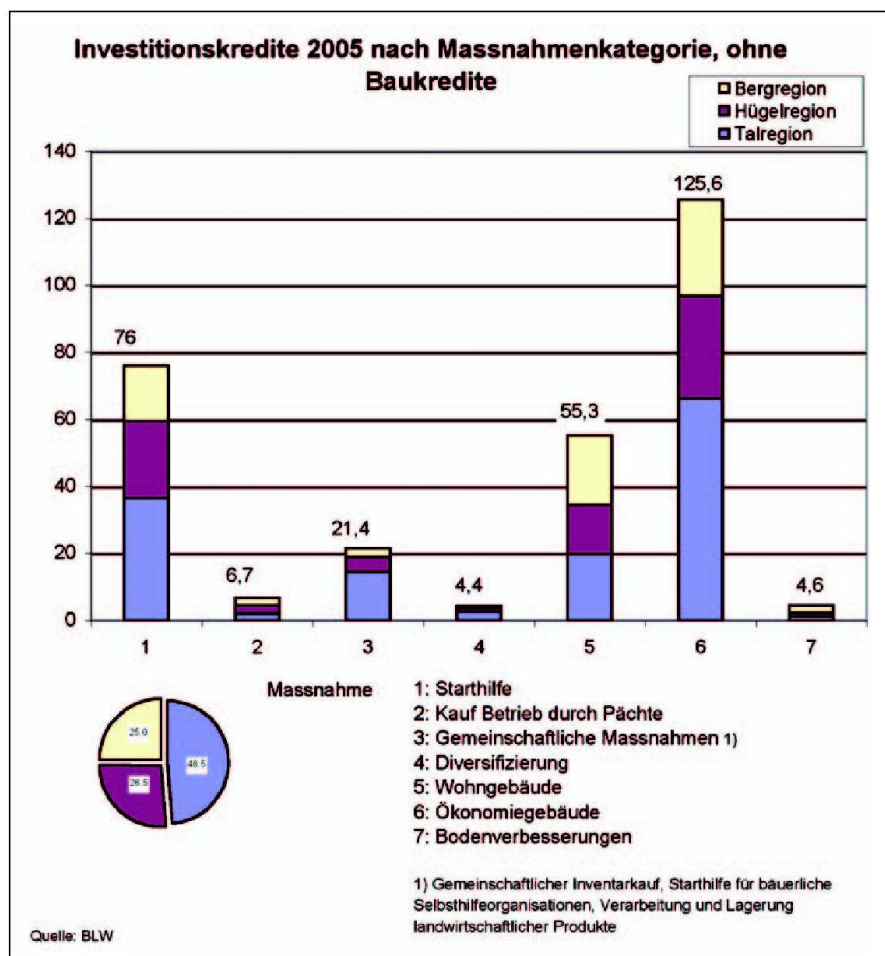
Abb. 3: Investitionskredite.
