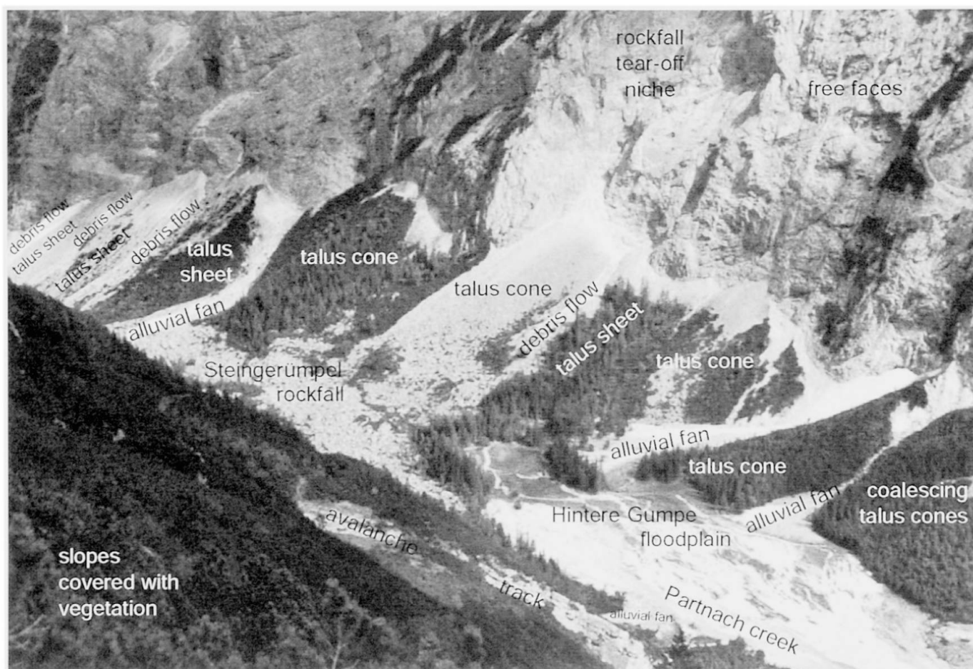
Fig. 2: Alpine landform assemblage around the Hintere Gumpe floodplain (Reintal, Bavarian Alps). Photo overlaid with labels of landforms, view facing south-east.
