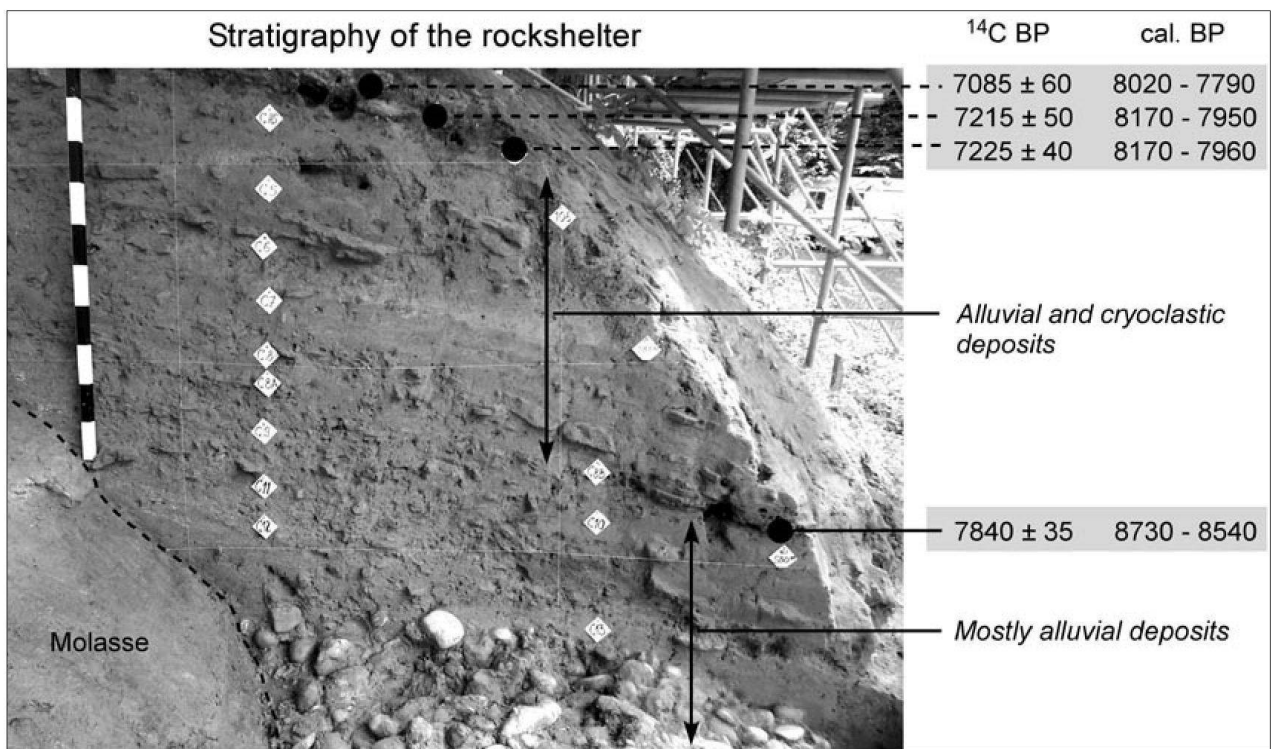
Fig. 7: Base of the infilling of the rockshelter and results of the radiocarbon dating of charcoal and bones found in the archaeological layers
