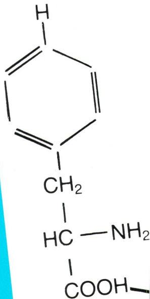
Phenylalanin
