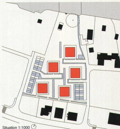
Situation 1:1000
