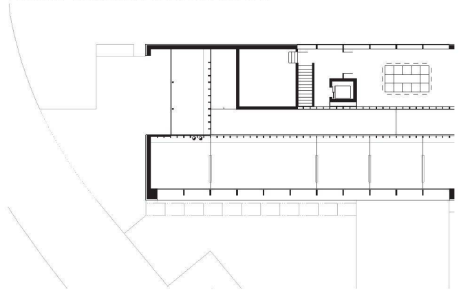
✓Grundriss Erdgeschoss. ✓Floor plan: ground floor.
