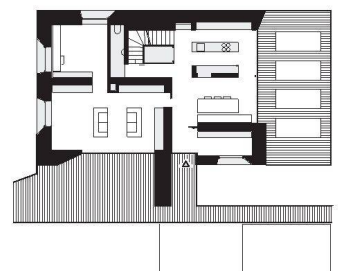
Erdegessch | Ground floor
