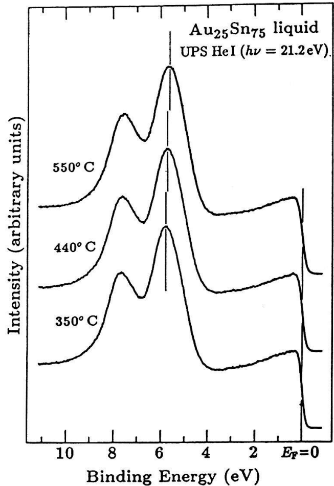
Fig. 1b: UPS HeI spectra of liquid \text{Au}_{25}\text{Sn}_{75} at different temperatures.
