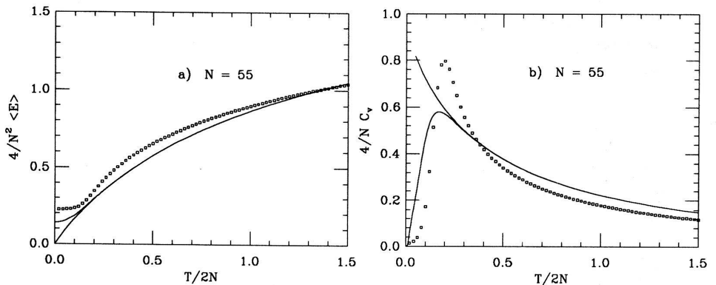
Fig. 2 Normalized mean energy (a) and specific heat (b) vs. normalized temperature obtained from exact enumeration of the skew-symmetric configuration space (square symbol). The curves represent the finite chain result. The finite value of the energy and the peak in the specific heat are due to the low energy cut off.
