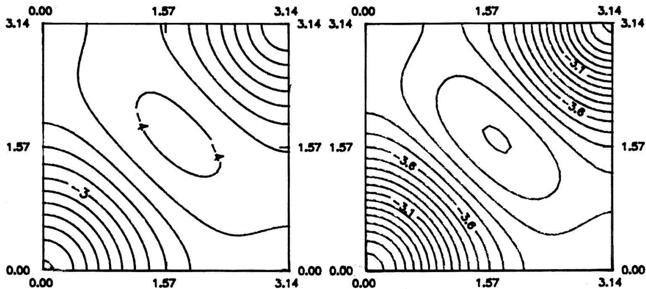
Fig.2 Equienergetic lines e(\vec{k}) = \text{const} ( \tau = 1 ) for direct O - O hopping h = 0.3 . a) Without frustration, \alpha = 0 . b) For \alpha = 0.2 .
