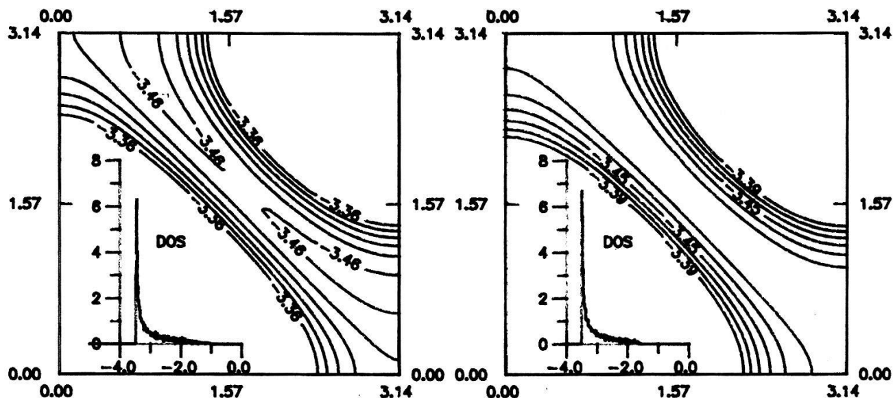
Fig.1 Equienergetic lines e(\vec{k}) = \text{const} , O - O hopping via Cu \tau = 1 , direct hopping h = 0 . a) Without frustration, \alpha = 0 . b) For \alpha = 0.2 . Density of states is plotted in the inserts.
