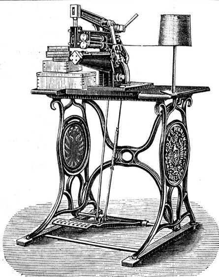
Cartonheftmaschine.
