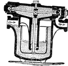
Condensationstopf
