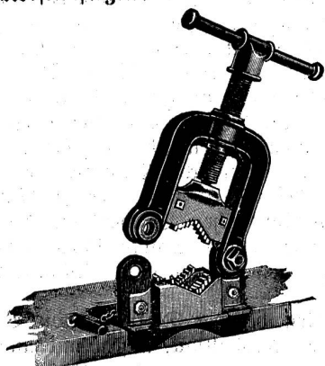
Fig. 1. Reed's Rohr-Schraubstock.
