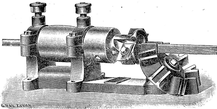
Rundstabhobelmaschine
