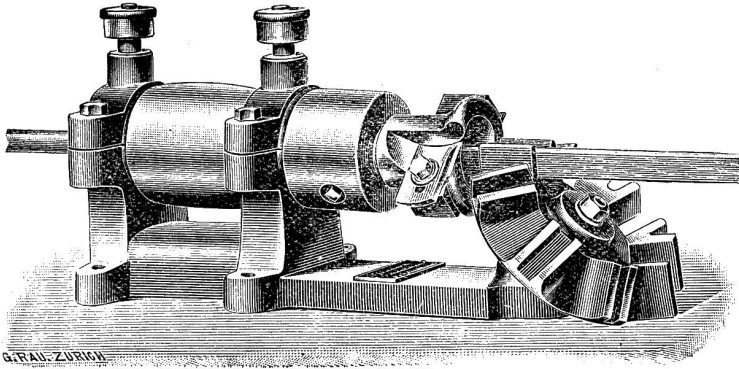
Rundstabhobelmaschine
