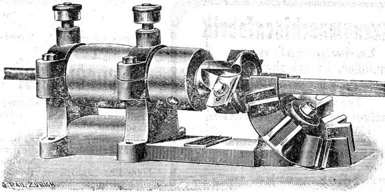
Rundstabhobelmaschine
