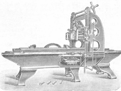
Hobel-Maschine.
