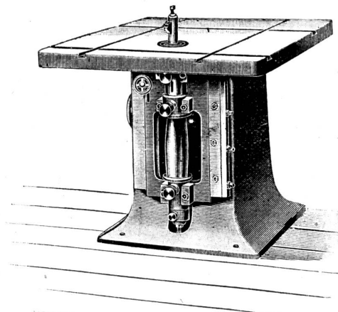
Kehlmaschine.
