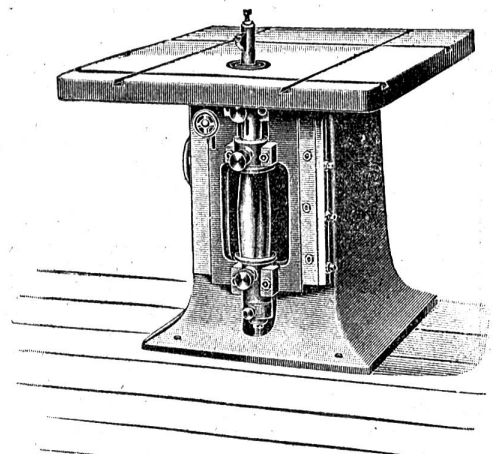
Kehlmaschine.
