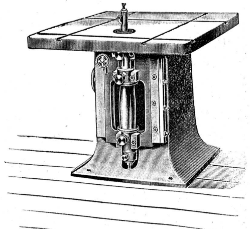
Kehlmaschine.
