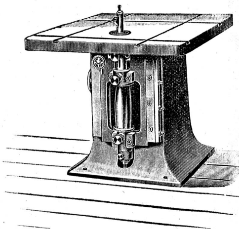
Kehlmaschine.
