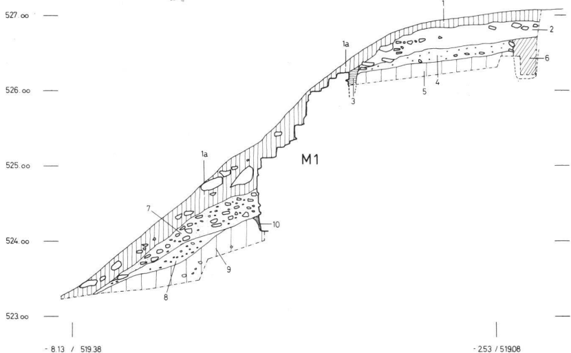
Füllinsdorf Altenberg 1982 Profil P13/14 in F8/F9, M 1:20
