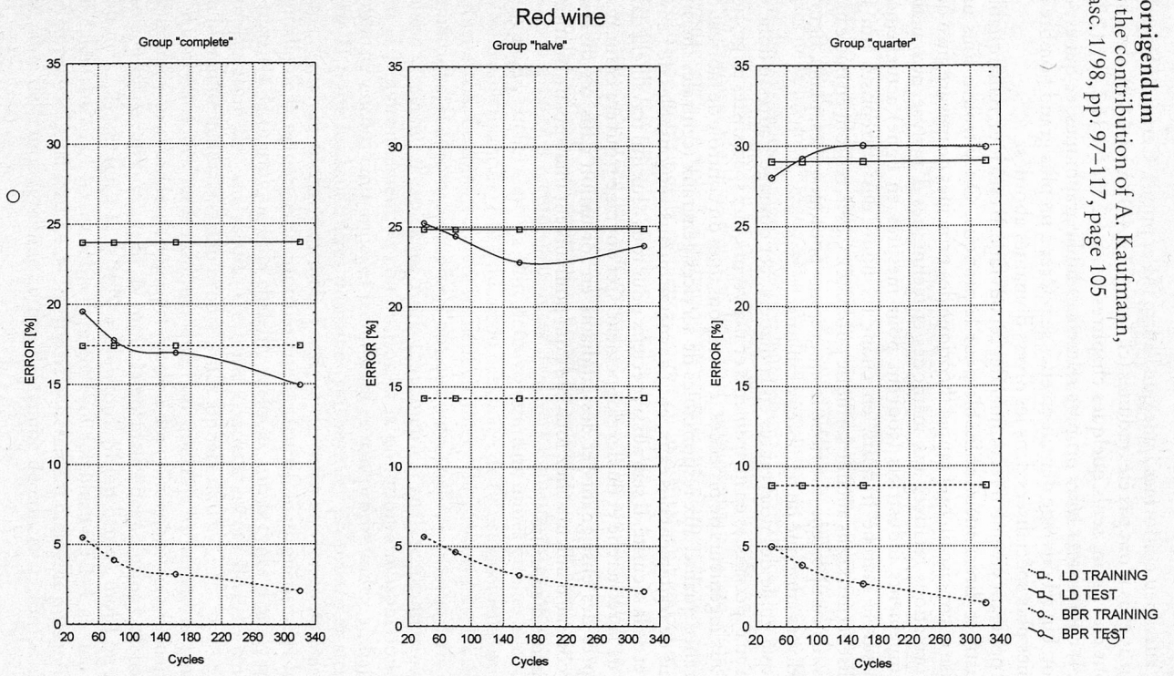
Fig. 3. Red wines originating from nine different geographical origins were classified. The figure is otherwise equivalent to figure 2. Again, using less training samples (complete, halve and quarter) increases the classification error of unknown test samples. There is no clear difference between neural networks and discriminant analysis. Neural networks build by using limited training samples «quarter» should not be overtrained by performing too many iterations.
