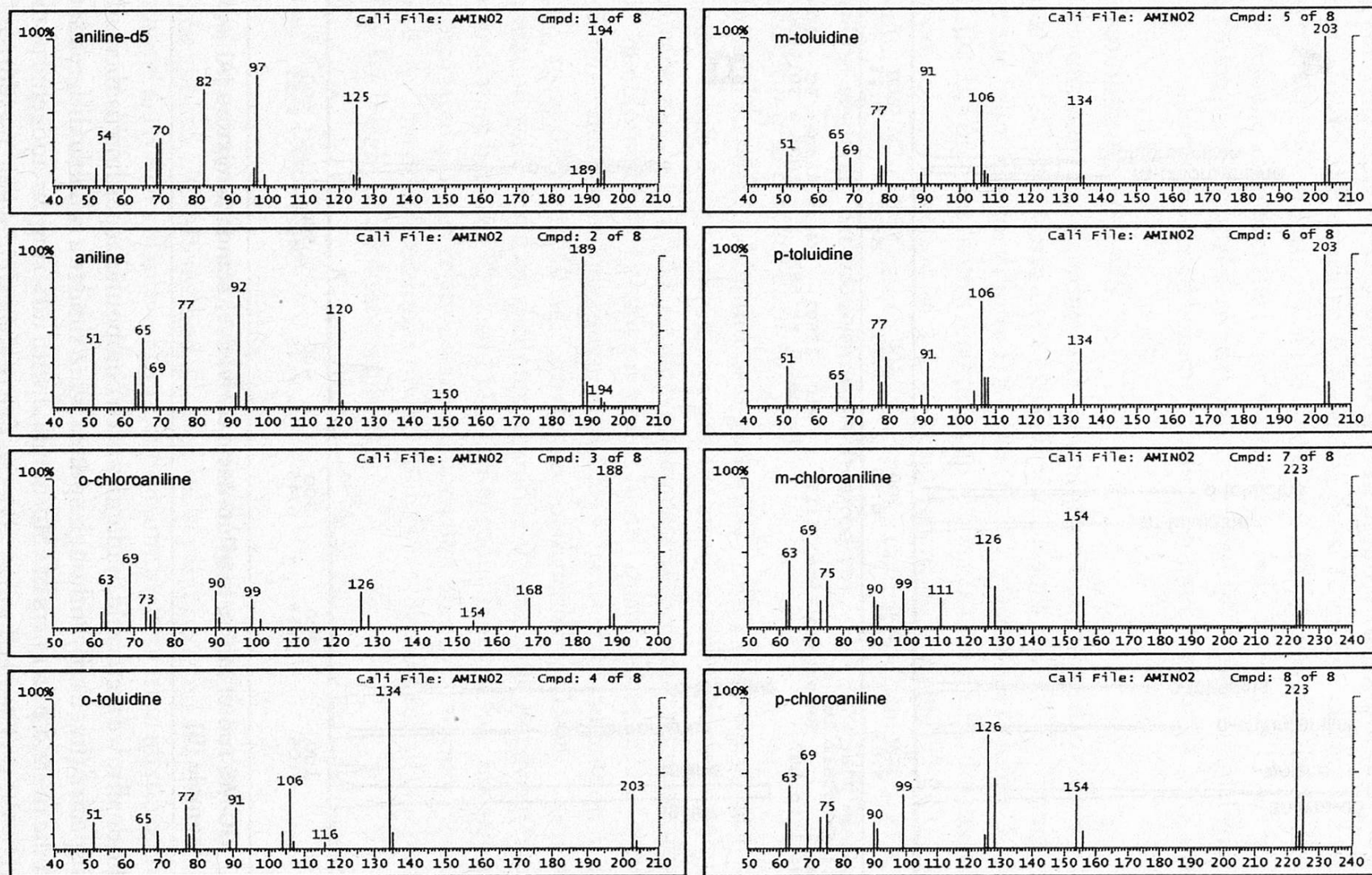
Figure 2 MS spectra of amine standards (perfluoroacyl derivatives)
