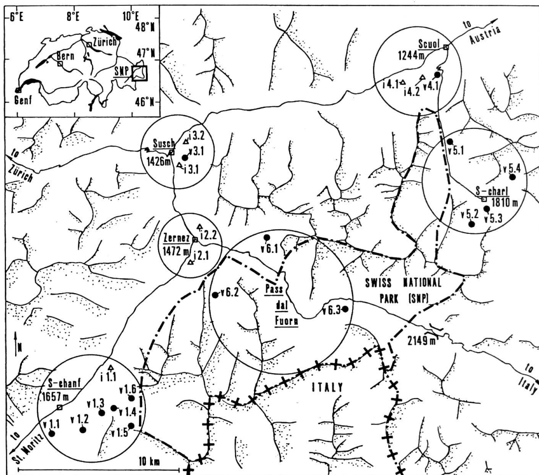
Figure 1: Locations of Alnus incana (i) and A. viridis (v) in the six regions of the Swiss National Park visited by Favre (see Table 1 for locations).
