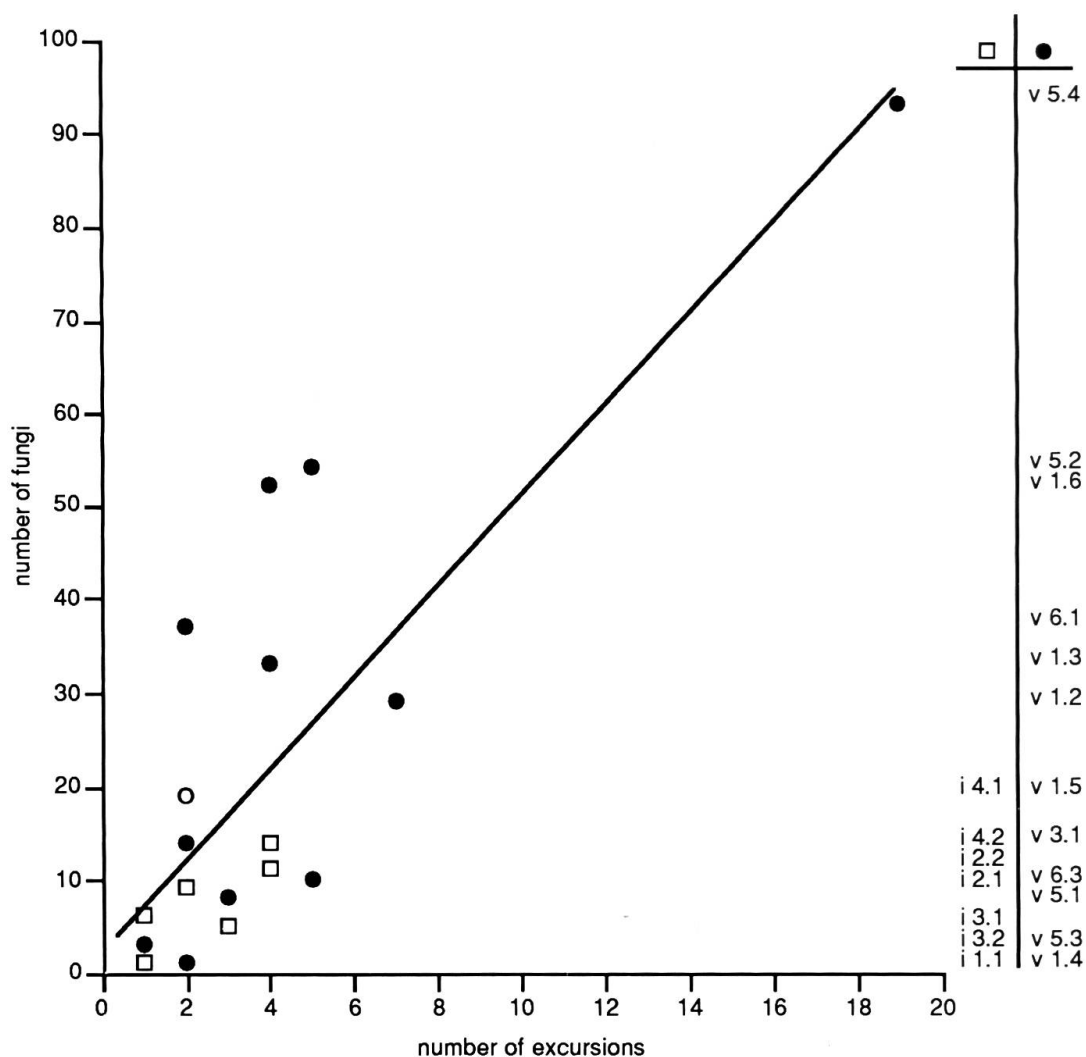
Figure 2: Relation between Favre's number of excursions and number of species of fungi (see Table 1 for locations). No excursion were noted in the field books to the locations v 1.1, v 4.1, and v 6.2.
