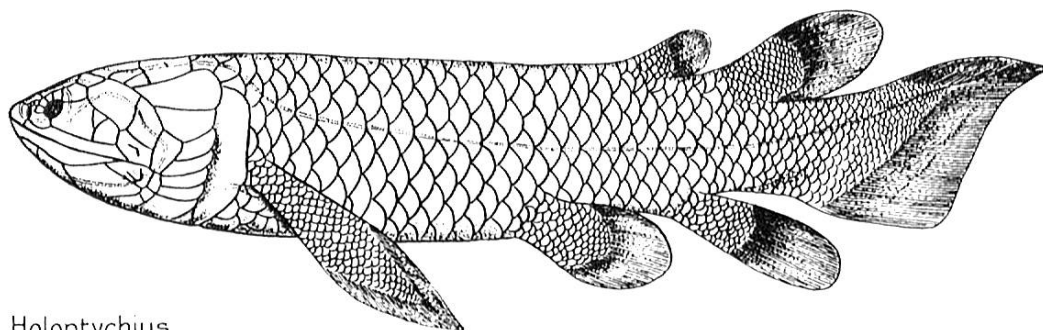
Holoptychius
