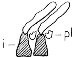
Crossopterygier
