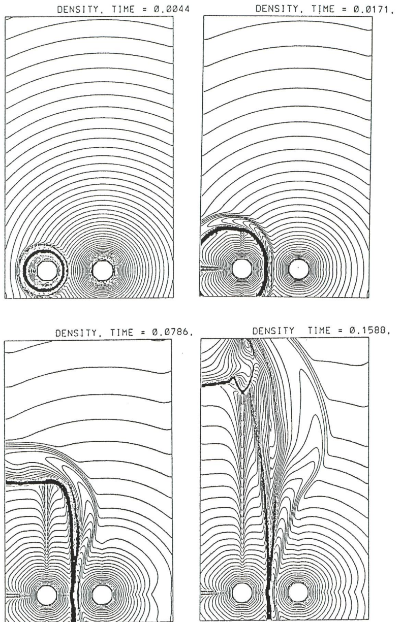
Colliding winds
