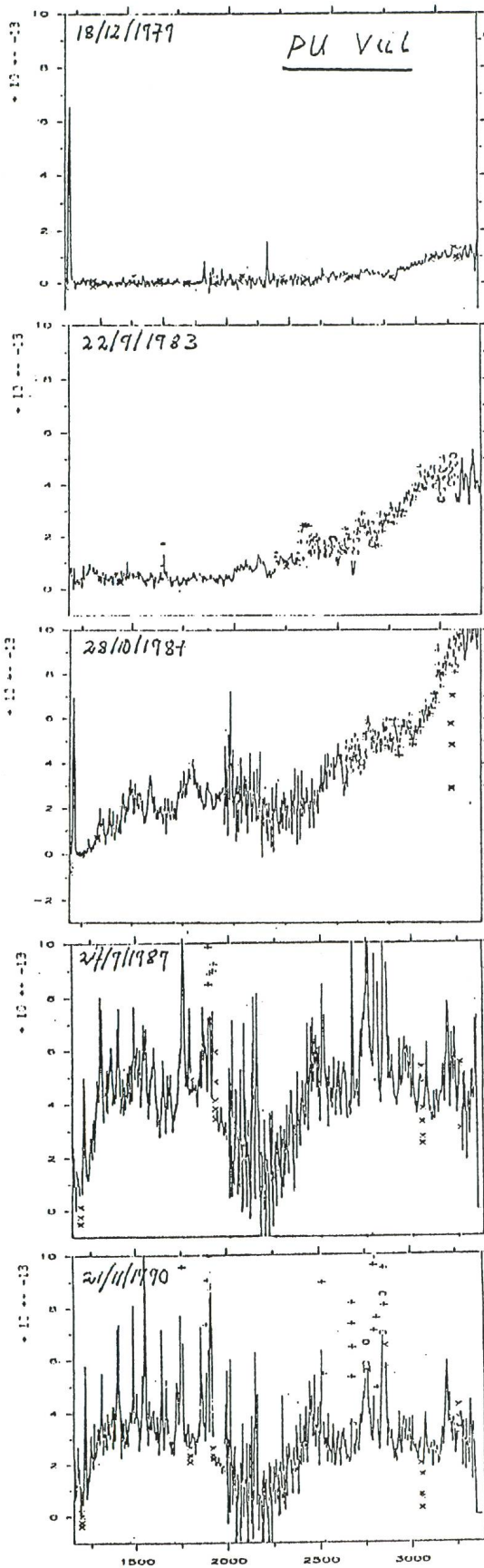
Colliding winds
