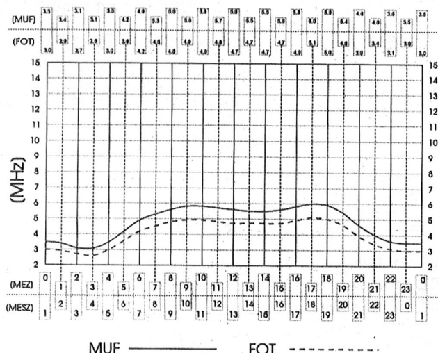
Bern September 1996 R = 6
