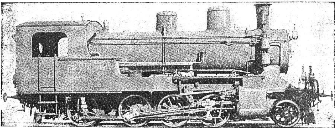
\frac{1}{3} Heissdampflokomotive.
